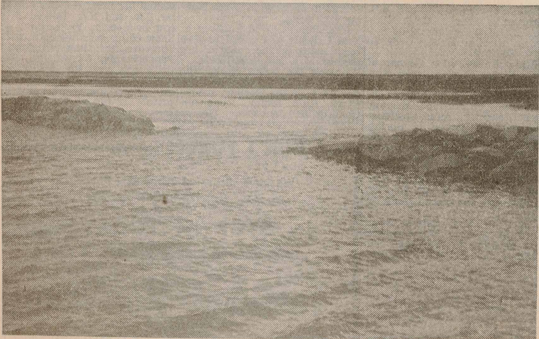
(Cape Cod Standard-Times Photo) This is the Provincetown Harbor West End breakwater, which Army Engineers will repair. Shown in this picture, taken from the West End traffic circle, is the breakwater, with the break in the structure, nearest the shore, depicting water pouring through on a rising tide. The water pours through this gap, and several other gaps, with a terrific speed, both on incoming and outgoing tides. During the Summer, unsuspecting visitors wander out and are stranded.
